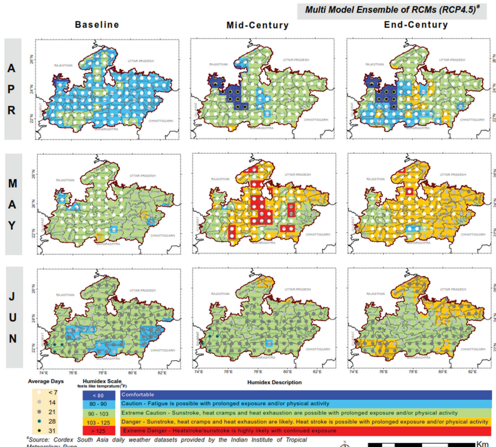
Figure 21 : Humidex projections for Madhya Pradesh
