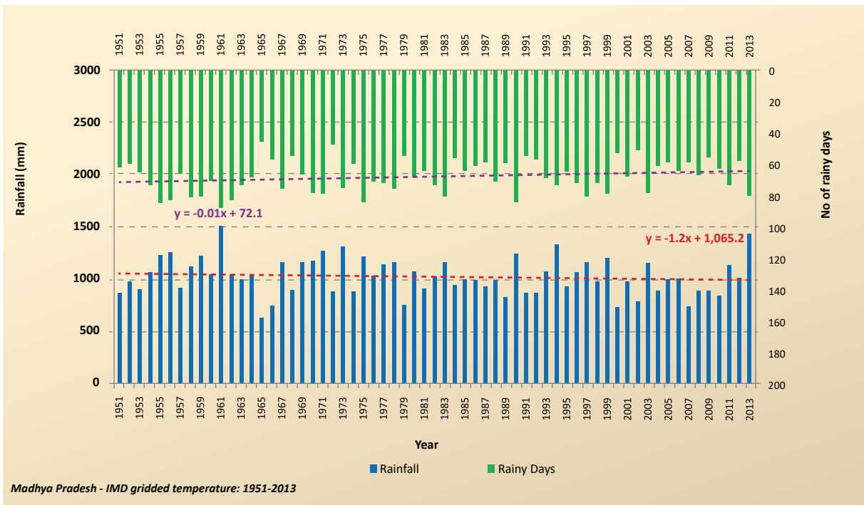
Figure 11 : Characteristics of observed annual rainfall and number of rainy days for Madhya Pradesh
