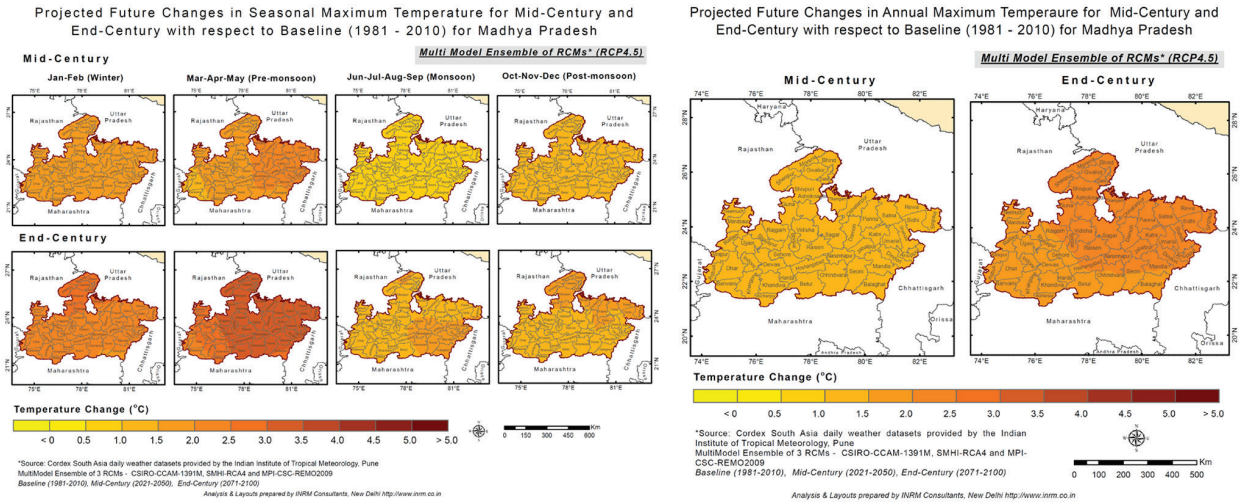
Figure 11 : Spatial representation of projected changes in annual and seasonal maximum temperature for IPCC AR5 RCP4.5 scenario
