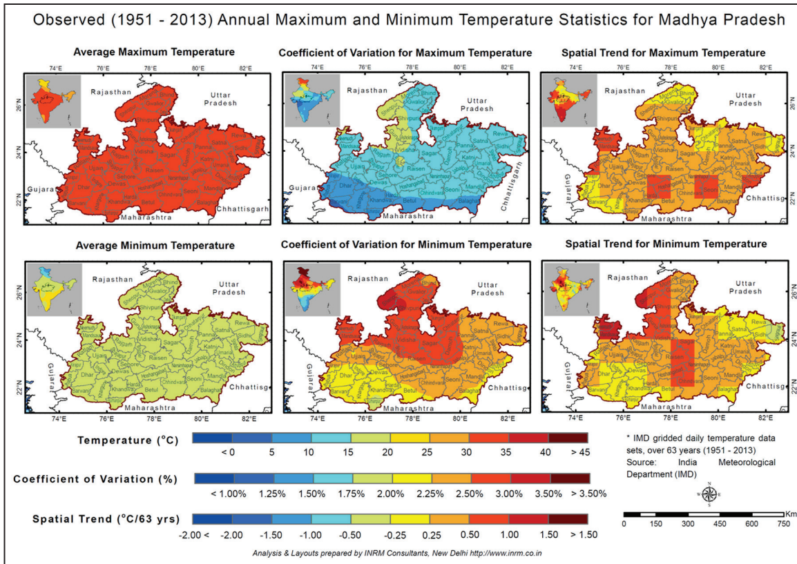
Figure 9 : Spatial variation in observed average annual and seasonal maximum and minimum temperature for Madhya Pradesh (1951-2013)
