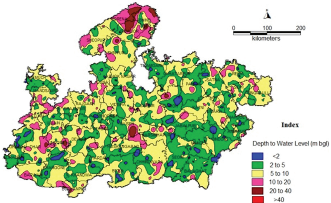
Depth to Water Level Map of Madhya Pradesh (Jan-2020)
