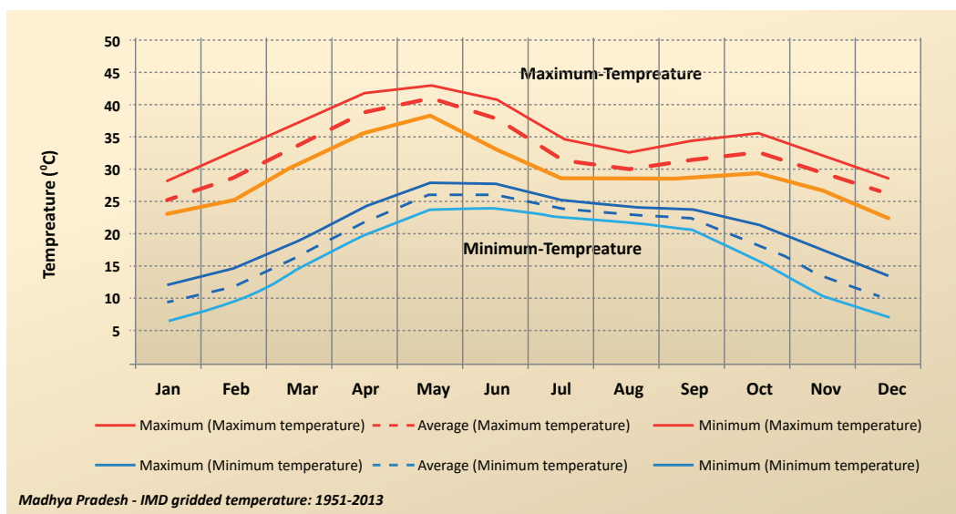
Figure 8 : Long term monthly average, maximum and minimum temperature for Madhya Pradesh(1951-2013)
