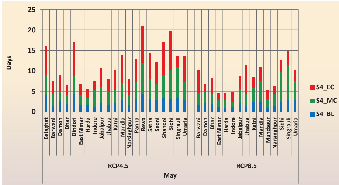
Figure 21 : Humidex projections for Madhya Pradesh
