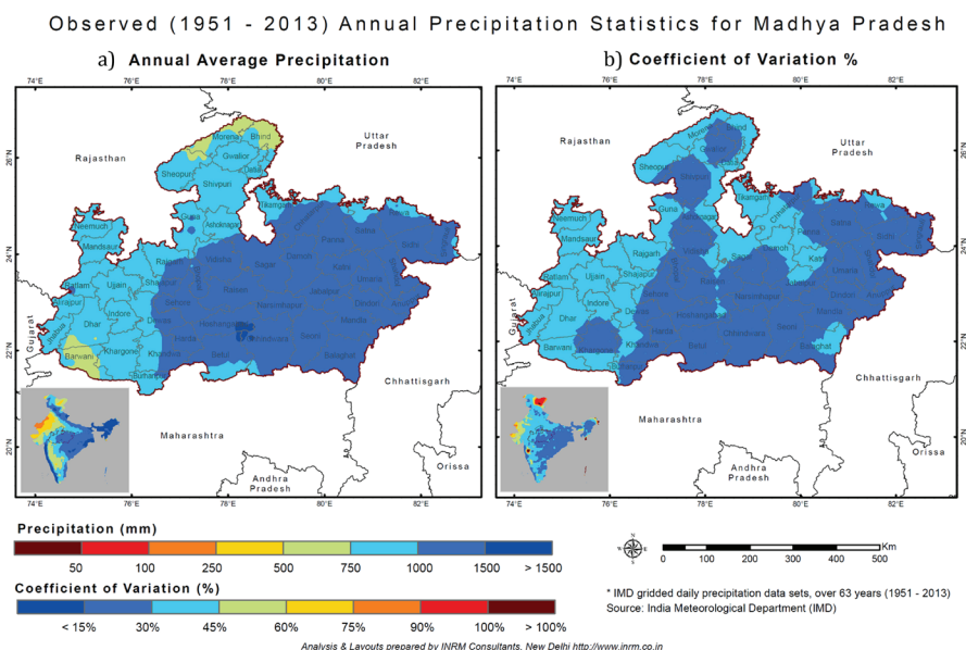
Figure 10 : Spatial variation in observed average annual and seasonal rainfall for Madhya Pradesh (1951-2013)
