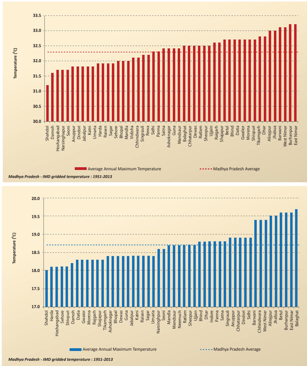
Figure 7 : Long term annual average, max and min temperature for districts of Madhya Pradesh (1951-2013)
