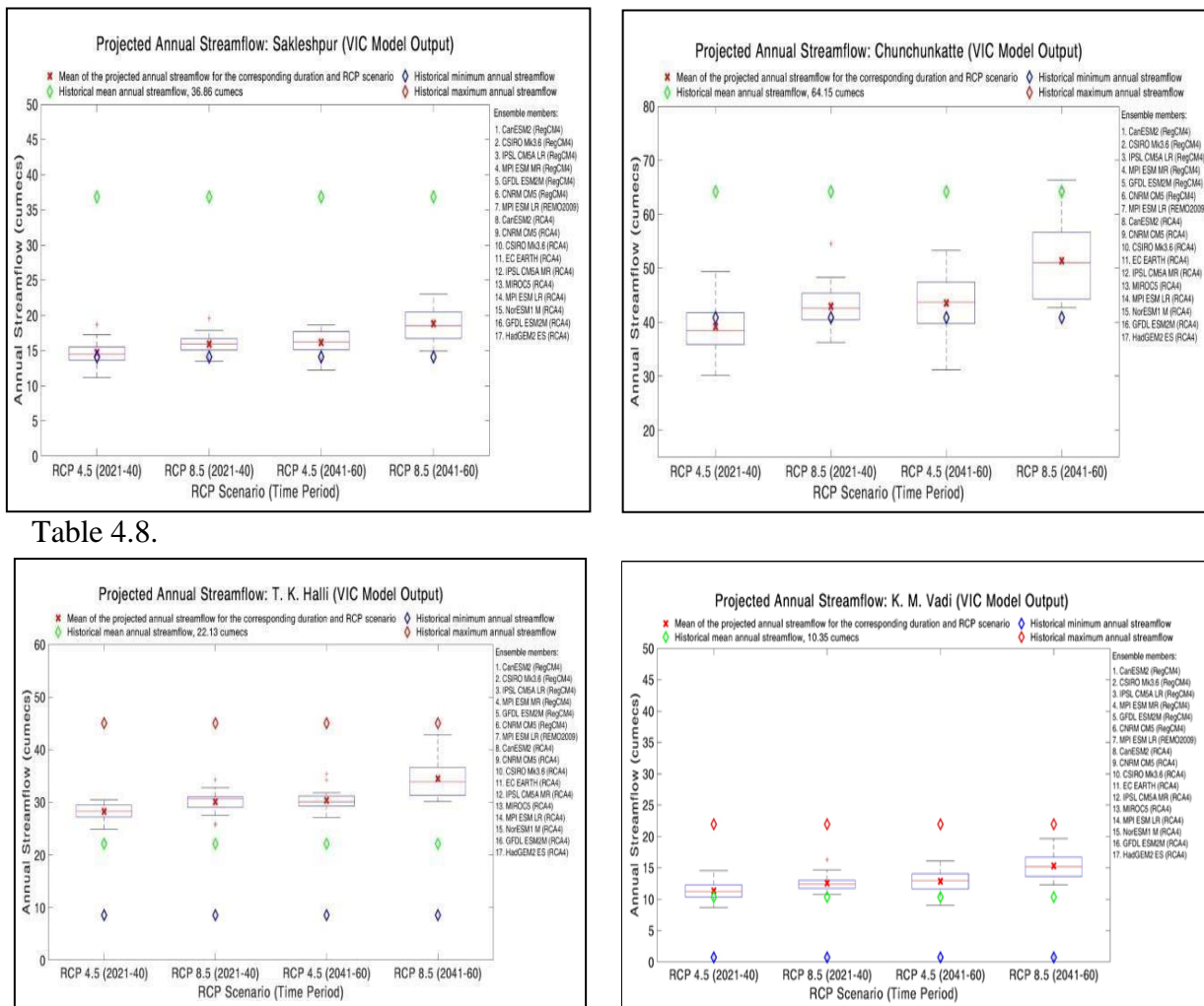
Figure 4.11: Projected ensemble averaged annual streamflow (cumecs) at a) Sakleshpur b) Chunchunkatte c) K. M. Vadi d) T.K. Halli e) Kollegal stations in the Upper Cauvery basin
